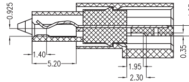
SECT C-C
