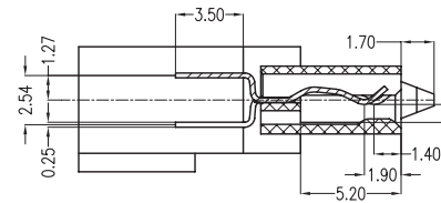
SECT B-B
